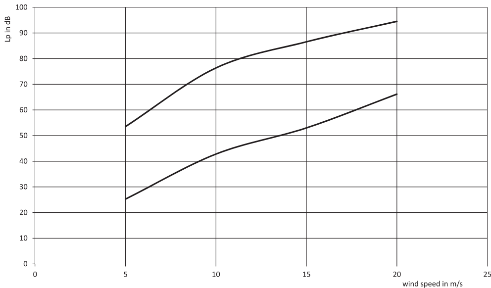
level of wind generated noise with and without windscreen Terz 250 Hz
